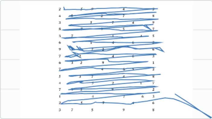
DEM Test C eye trace Combined eye trace
